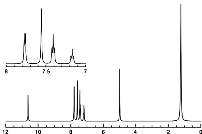
Figure 3. 1 H NMR spectrum of 5a with all aromatic protons resolved.
