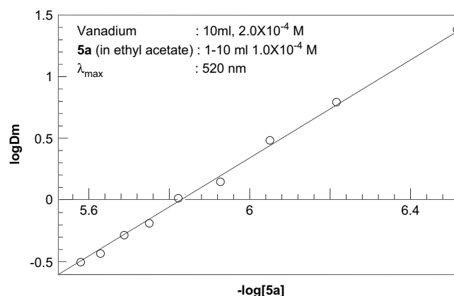
Figure 4. Slope ratio plot for determination of stoichiometry of vanadate complex of 5a .
